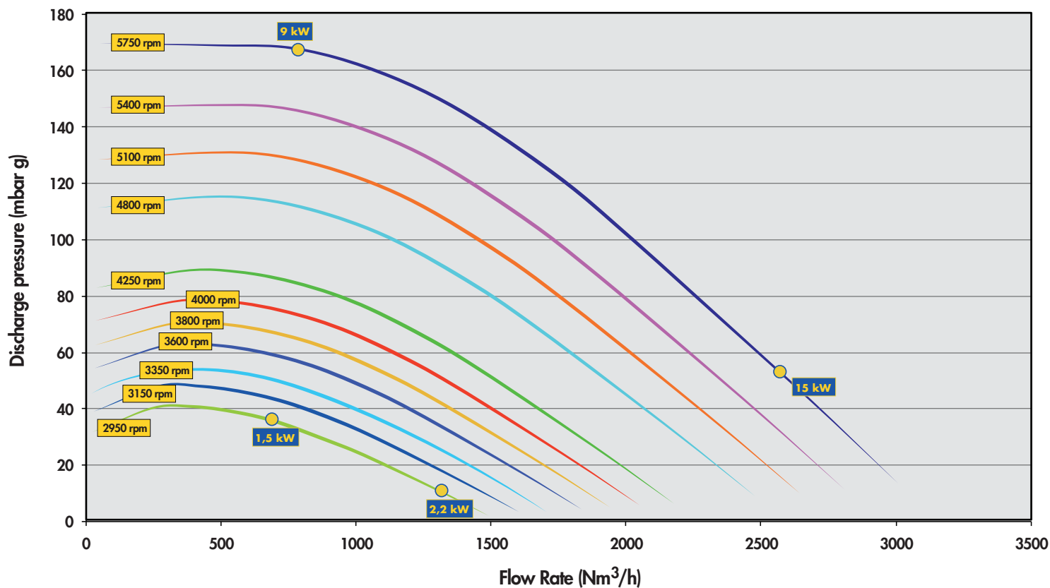
GB100VB : Biogas pressure curve characteristic
